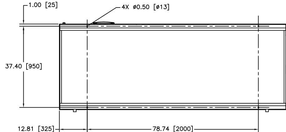
ANCHOR BOLT LOCATIONS
