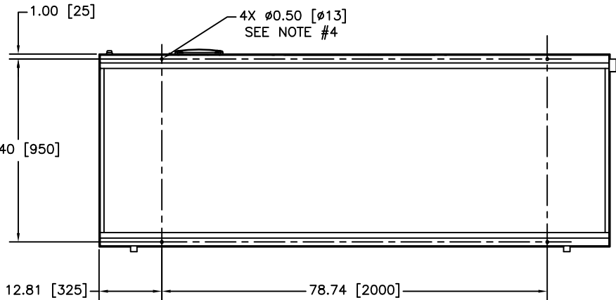
ANCHOR BOLT LOCATIONS & ISOLATOR MOUNTING
