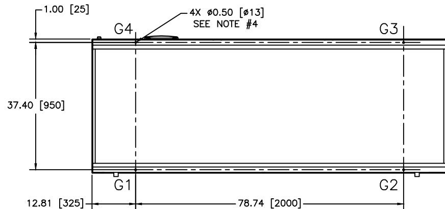
ANCHOR BOLT & ISOLATOR MOUNTING LOCATIONS
