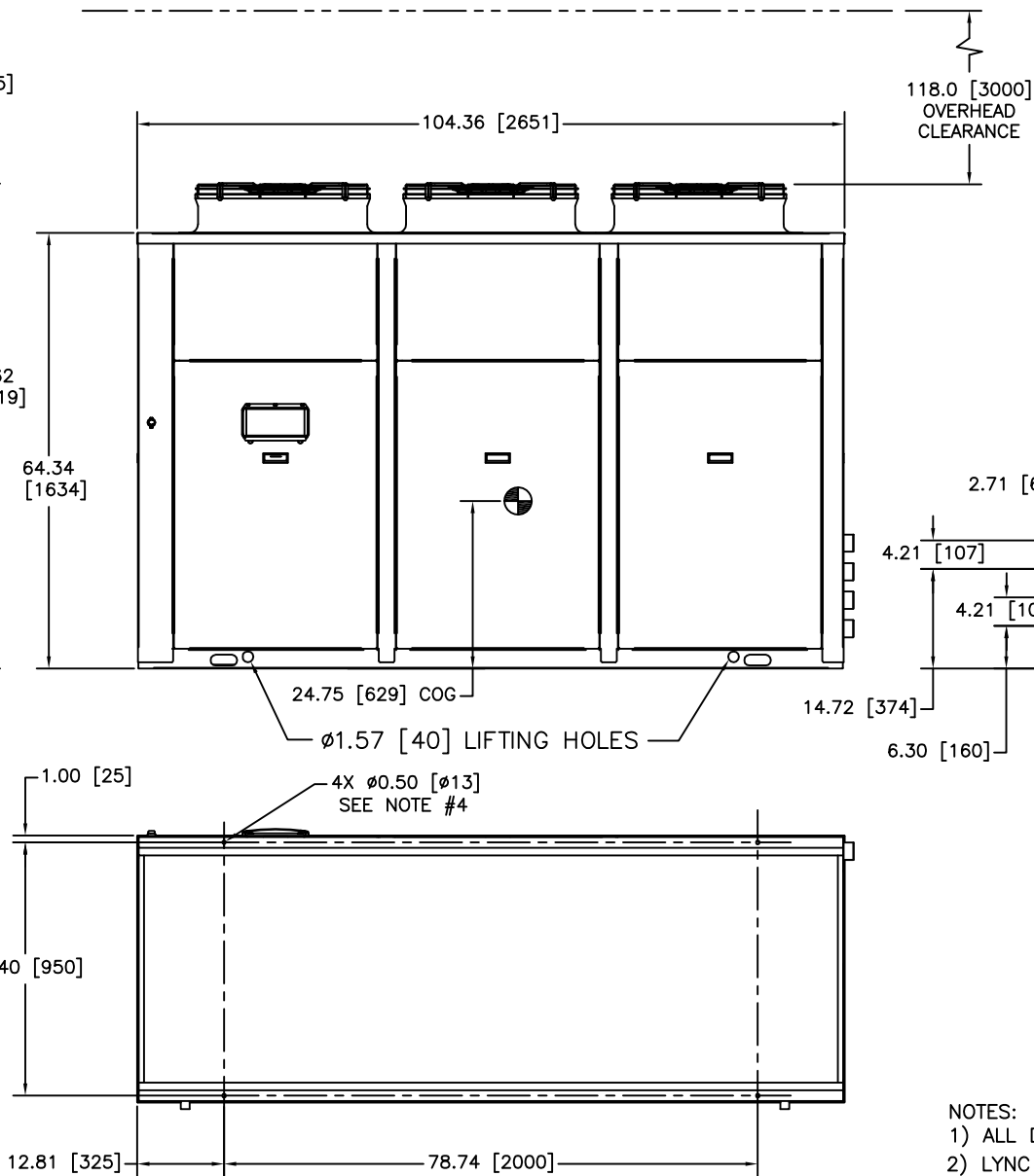
ANCHOR BOLT LOCATIONS & ISOLATOR MOUNTING
