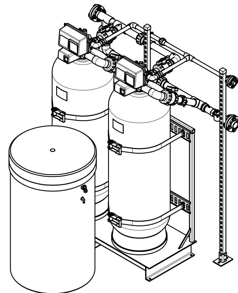
ISOMETRIC VIEW FOR REFERENCE ONLY
